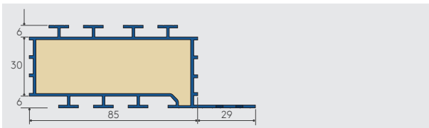
Figure 26: Kingspan Thermabate® 85
