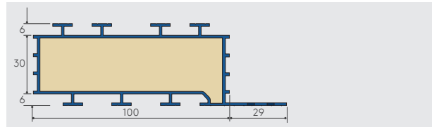
Figure 28: Kingspan Thermabate® 100
