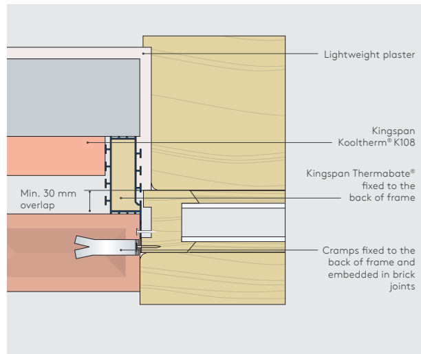
Figure 6: Window frame & Kingspan Thermabate® fitted as a combined unit
