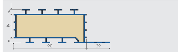
Figure 27: Kingspan Thermabate® 90
