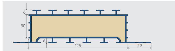
Figure 30: Kingspan Thermabate® 125
