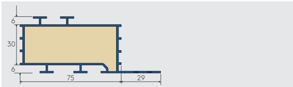
Figure 25: Kingspan Thermabate® 75
