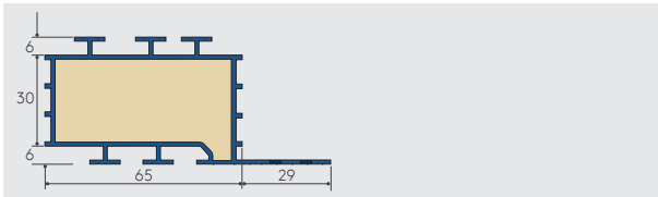
Figure 24: Kingspan Thermabate® 65
