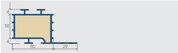
Figure 23: Kingspan Thermabate® 50
