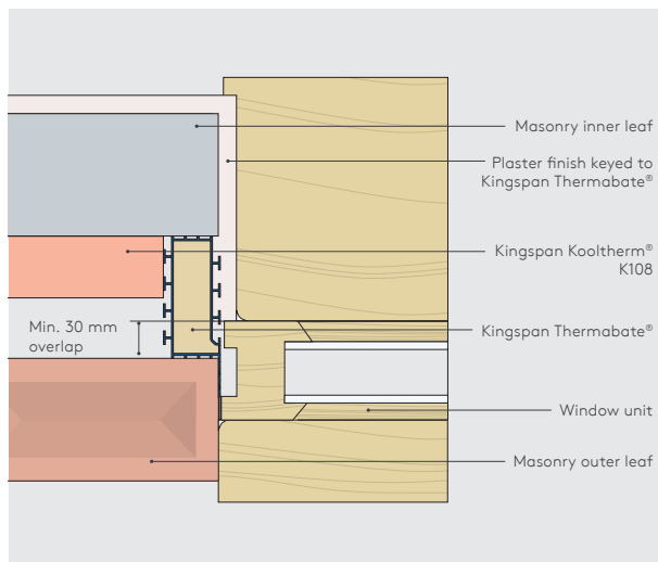
Figure 4: Flush reveal
