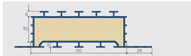
Figure 29: Kingspan Thermabate® 110
