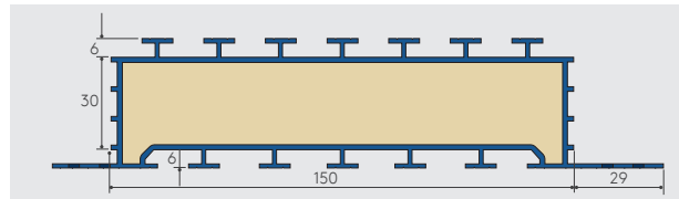
Figure 32: Kingspan Thermabate® 150
