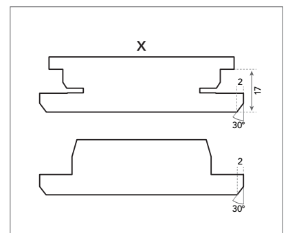
Concealed grid system with the symmetrical X edge tile ensuring quick installations in both directions.
